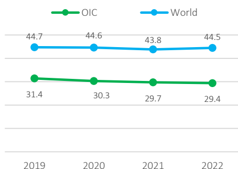
Proportion of Medium and High-tech Industry Value Added in Total Value Added (%)
