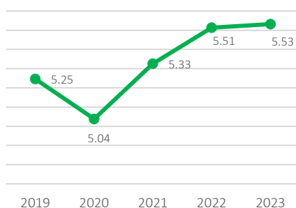
OIC Countries CO 2 Emissions, Territorial, Total (Billion Tonnes)
